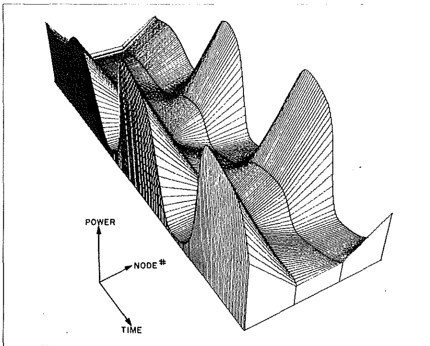
Above, Perspective view of the reactor power as a function of time at several reactor core locations.
