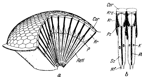
Figure 11. Structure of the compound eye of a fly (schematic): (a): Whole eye, from which a section is dissected on the right (according to Hesse) (b): Two ommatidia Cor: Chitincornea; K: nucleus; Kr: crystalline lens; Krz: lens cell; Nf: nerve fiber; P: pigment; Retl: retinula; Rh: rhabdom; Sz: visual cell
